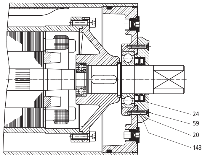
220M & 220H Stainless steel option TS10N & TS12N
