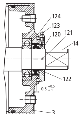
Labyrinth Option - Mild Steel
